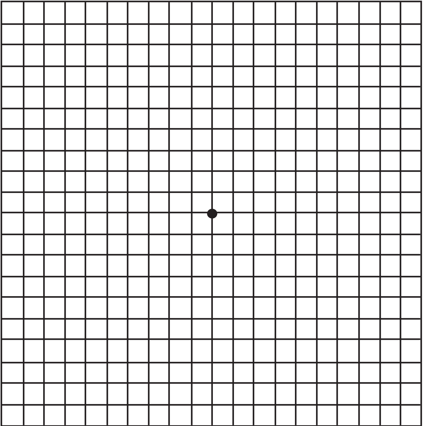
Amsler Grid
